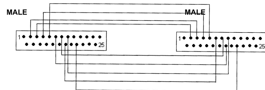
WIRING DIAGRAM
