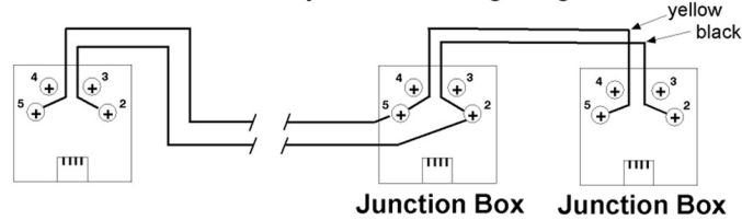
Junction Box "Daisy Chain" Wiring Diagram
